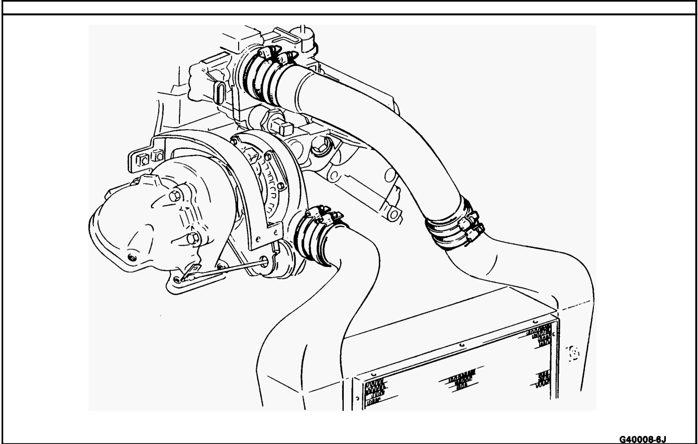
Figure 52 Intercooler to Engine
