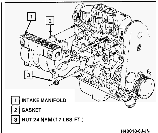
Figure 36 Intake Manifold
