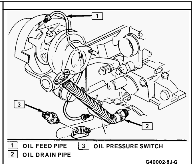
Figure 50 Oil Supply & Return Line Routing
