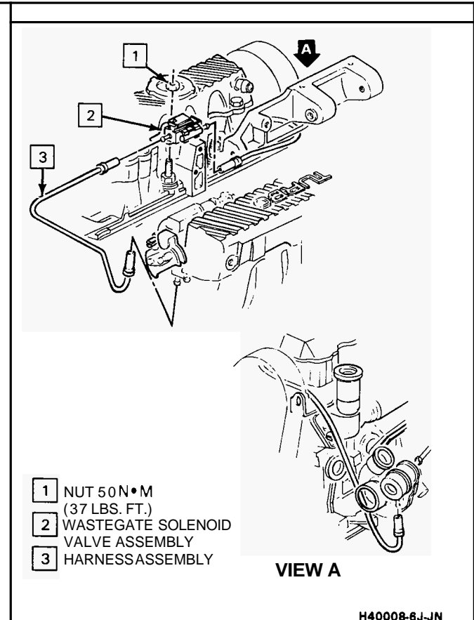
Figure 34 Wastegate Solenoid Valve Assembly & Harness
