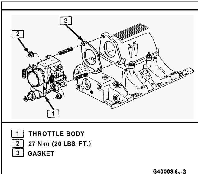
Figure 48 Throttle Body Attachment
