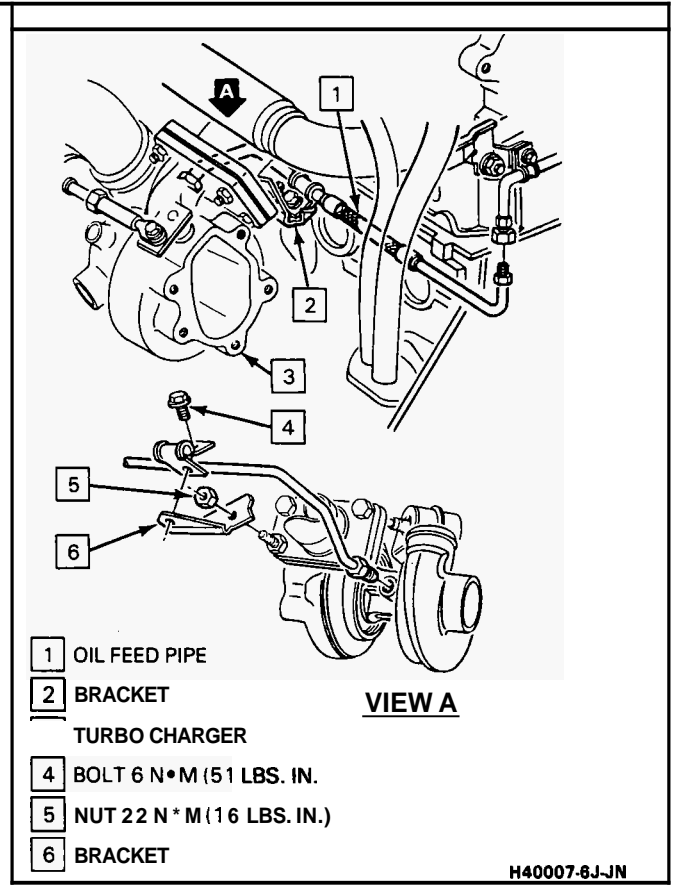
Figure 41 Turbo Oil Feed (LH)
