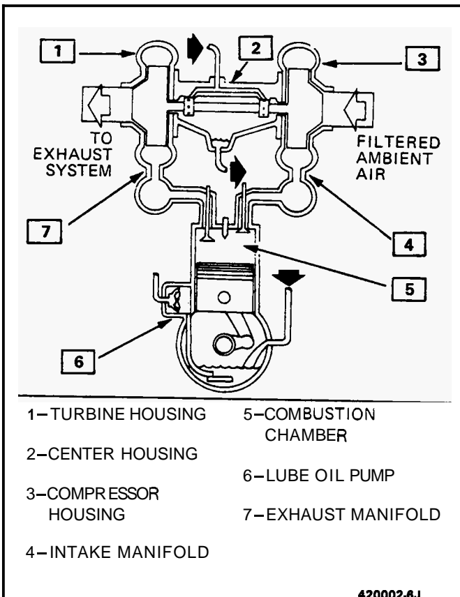
Figure 2 Turbocharger Operation
