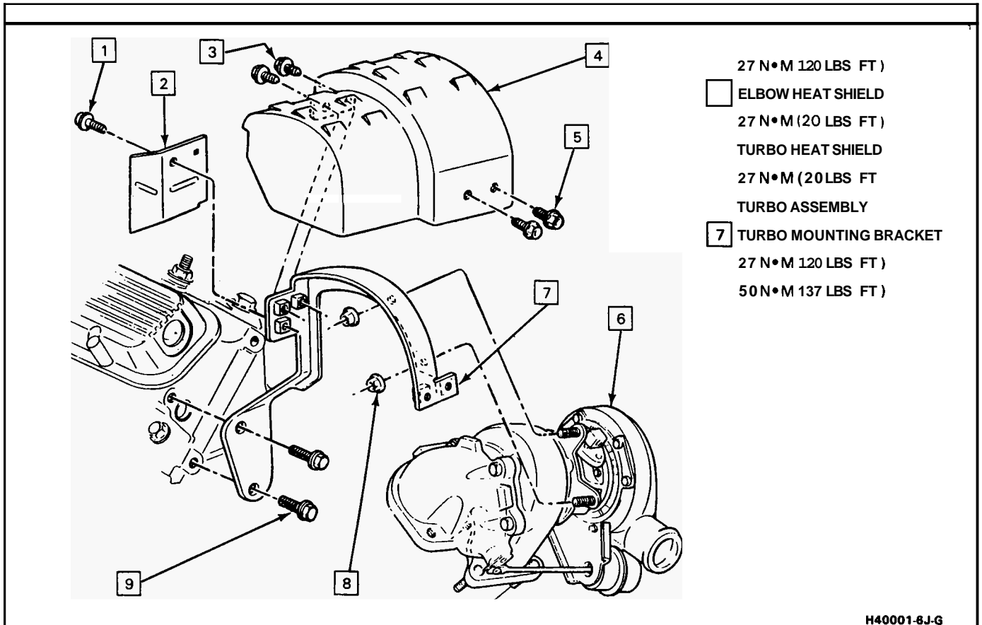
Figure 43 Turbocharger Assembly
