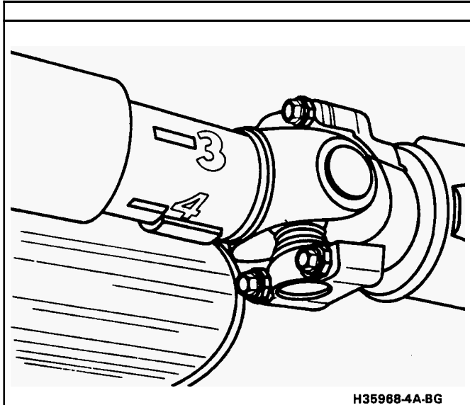
Figure 16 Reference Marks on Propeller Shaft
