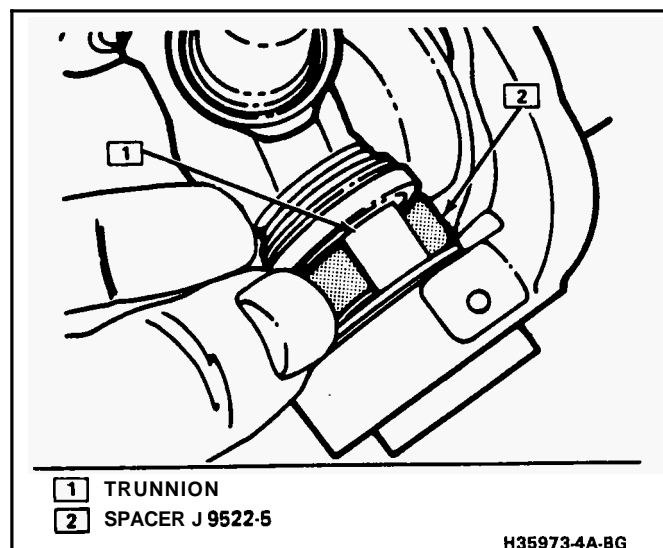
Figure 21 Using J 9522-5 Spacer
