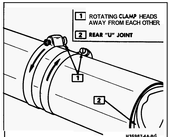
Figure 15 Rotating Balance Hose Clamps
