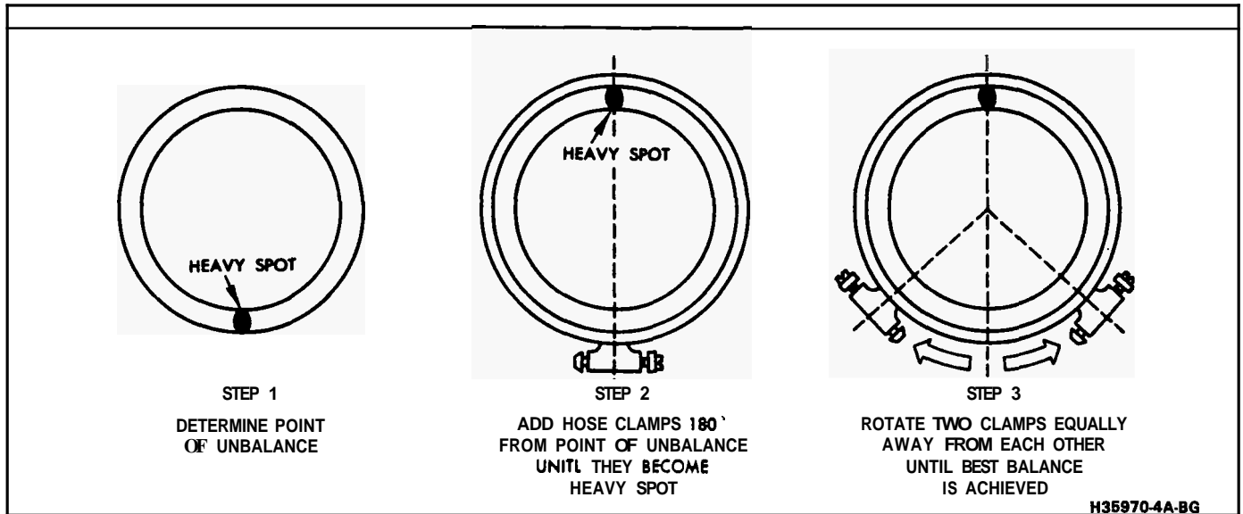
Figure 18 Positioning Hose Clamp to Achieve Best Balance
