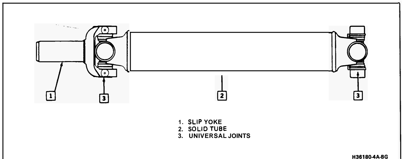
Figure 1 Propeller Shaft
